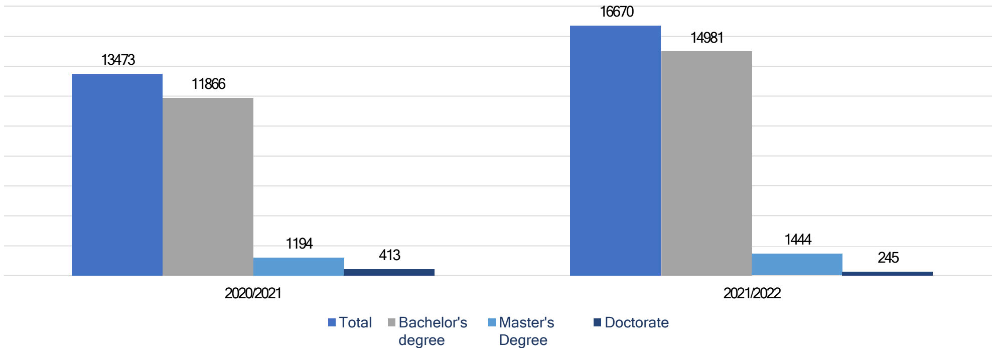
Student population 2020-2022
